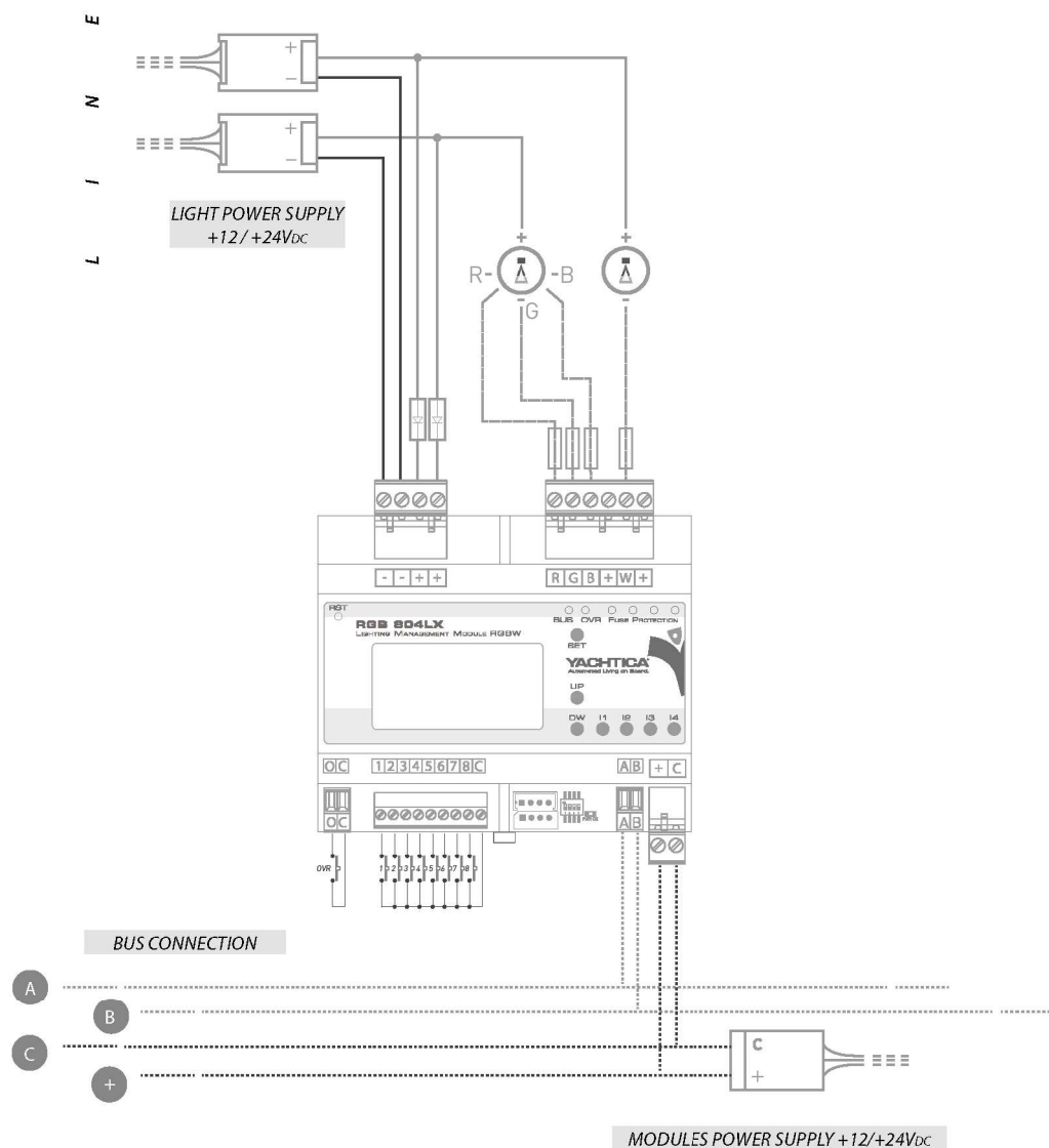
SCHEME 5: Wiring with direct positive with independent power supply (RGB + 1 W)(1 RGB + 1 W)
