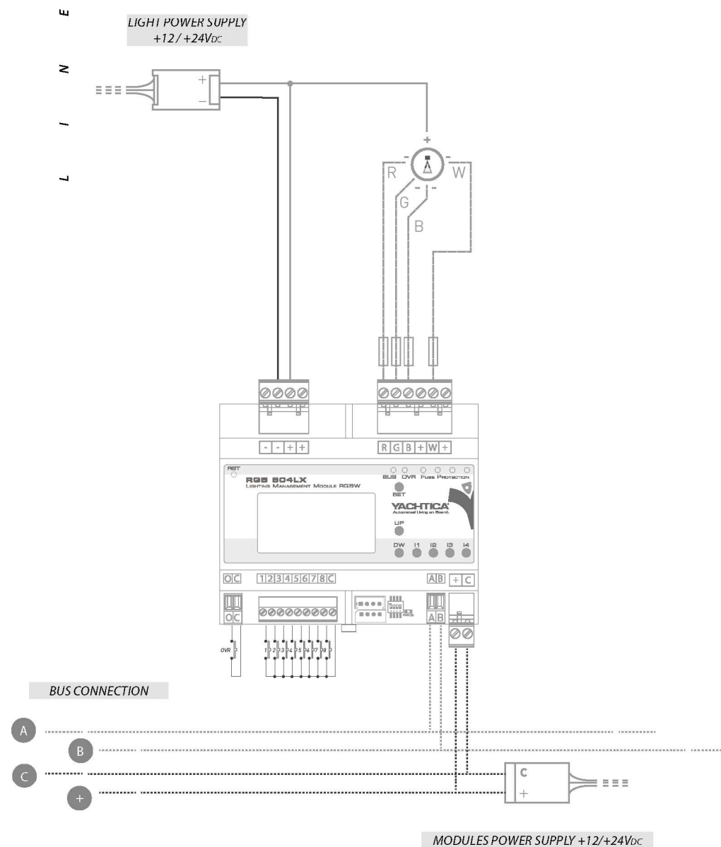
SCHEME 6: Wiring with direct positive (1 RGBW)
