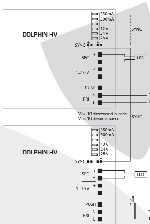
Schema con pulsante Diagram with push button
