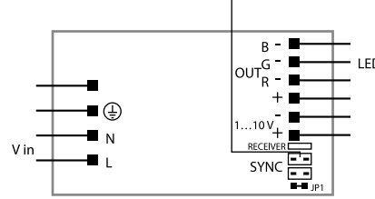
Schema - Diagram 16
