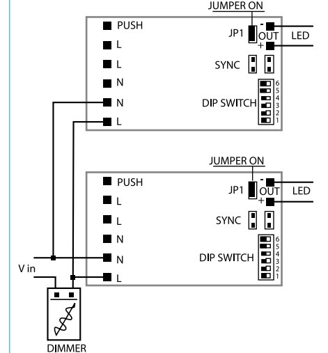
Schema - Diagram 5
