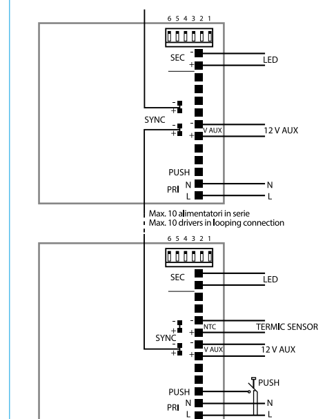
Schema - Diagram 8
