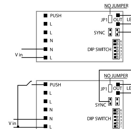
Schema - Diagram 6
